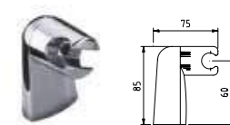
MADAGASCAR SOPORTE ARTICULADO Articulated holder Support douchette orientable
