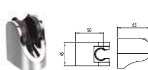
START SOPORTE ARTICULADO Articulated holder Support douchette orientable
