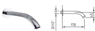
MIKURA 170 mm CAÑO MURAL Bath spout | Bec
