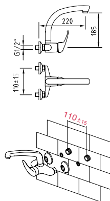
PANAM urban 185 mm
