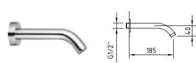
CAIMAN 185 mm CAÑO MURAL Bath spout | Bec
