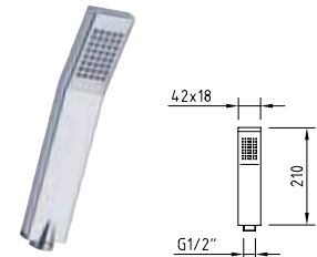
MARINA | 1F DUCHA | Handset | Douchette
