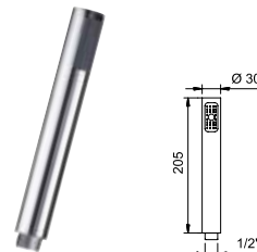
CAIMAN | 1F DUCHA | Handset | Douchette
