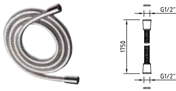
SILVER HOSE 1,75m FLEXIBLE | Flexible | Flexible
