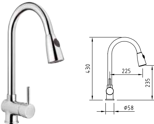
CAIMAN urban 235 mm
