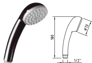
S12 | 1F | Ø70 mm DUCHA | Handset | Douchette
