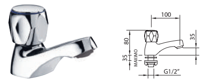
WITH2 guayama G180 ROBINET SIMPLE 35 / Single tap 35 Robinet, aérateur. Deck mounted single basin faucet, with aerator, cold water indice.
