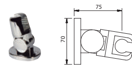
HABANA SUPPORT DOUCHETTE ORIENTABLE
