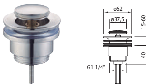
LYNX VIDAGE QUICK-CLAC Basin click waste
