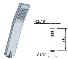
MARINA | 1F DOUCHETTE | Handset
