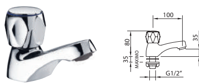
WITH2 guayama GMT ROBINET SIMPLE 35 / Single tap 35 Robinet, aérateur. Deck mounted single basin faucet, with aerator, cold water indice.
