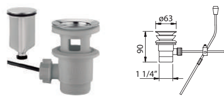
SYNTHÉTIQUE Synthetic - Pop-up waste
