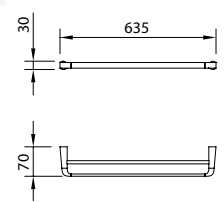
PORTE-SERVIETTE DOUBLE-BARRE Double towel rail
