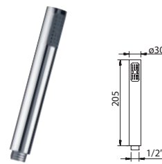
CAIMAN | 1F DOUCHETTE | Handset
