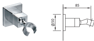
PASCUA SUPPORT DOUCHETTE ORIENTABLE
