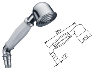
ANTIGONA | 1F | Ø50 mm DOUCHETTE | Handset
