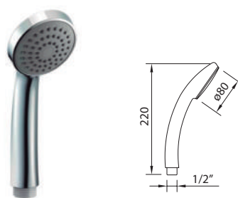
NF | 1F | Ø80 mm DOUCHETTE | Handset
