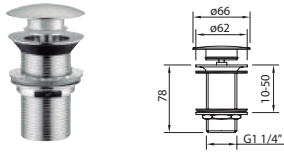
VELA VIDAGE QUICK-CLAC Basin click waste
