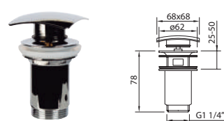
HYDRA VIDAGE QUICK-CLAC LAITON Basin click waste
