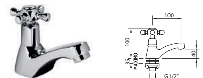
WITH2 antigona ROBINET SIMPLE 40 / Single tap 40 Robinet, aérateur. Deck mounted single basin tap, with aerator.
