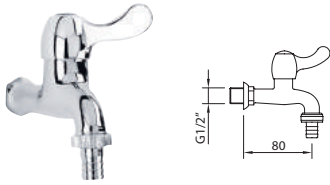
LAVE-MAIN / ROBINET JARDIN Sink and washing-machine tap Robinet, aérateur. Raccord pour tuyau. Wall mounted single tap. Hose fitting.
