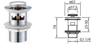
ORION VIDAGE QUICK-CLAC Basin click waste
