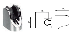
START SUPPORT DOUCHETTE ORIENTABLE
