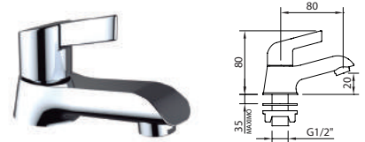
START elegance LAVE-MAIN / Single washbain tap Robinet, aérateur. Deck mounted single basin tap, with aerator.
