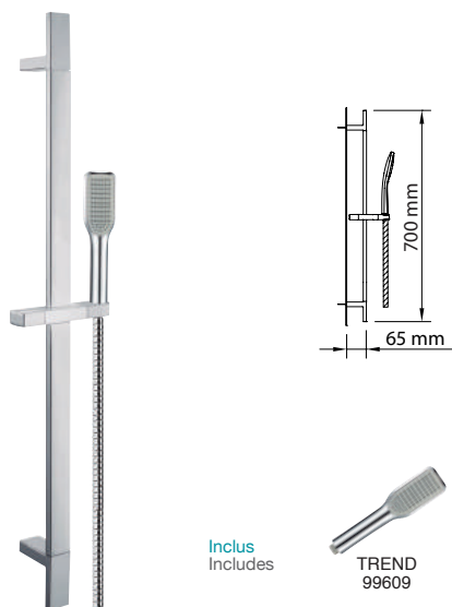
TREND - 30x10x700 mm ENSEMBLE BARRE DE DOUCHE Sliding bar set ABS
