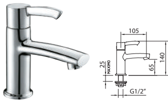
DESIGN LAVE-MAIN / Single washbain tap Robinet, aérateur. Deck mounted single basin tap, with aerator.
