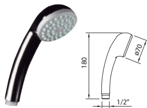
S12 | 1F | Ø70 mm DOUCHETTE | Handset
