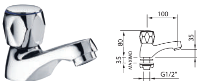
WITH2 guayama ROBINET SIMPLE 35 / Single tap 35 Robinet, aérateur. Deck mounted single basin faucet, with aerator, cold water indice.
