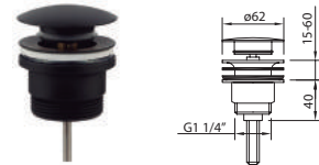
LEO NEGRO MATE VIDAGE QUICK-CLAC Basin click waste
