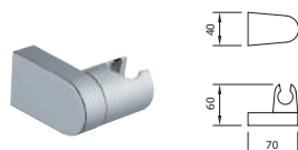
HABANA XTREME SUPPORT DOUCHETTE ORIENTABLE
