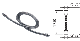
FLEXIBLE | Flexible 1,75m
