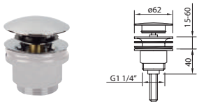
LEO VIDAGE QUICK-CLAC Basin click waste
