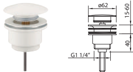
LEO BLANCO MATE VIDAGE QUICK-CLAC Basin click waste
